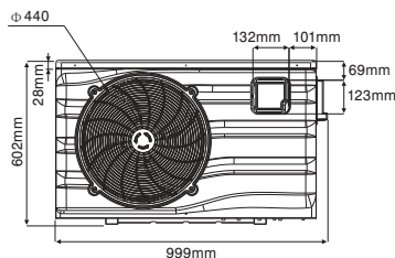
OASIS X9/X13 dimensions
