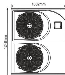
OASIS X28/X28T dimensions
